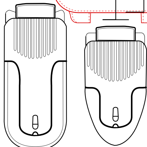
removable belt clip mechanism (front)
